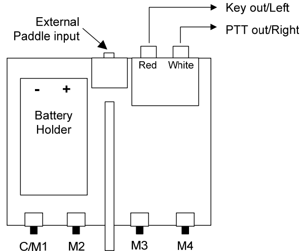
Figure 28 - PaddleStick Connection Diagram
