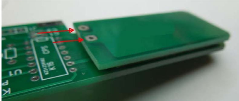
Figure 7 – Assemble paddle halves
