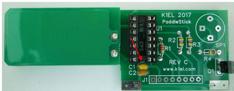
Figure 11 – Install socket, R's, C's, and Q1
