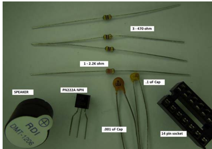
Figure 10 - PaddleStick board components
