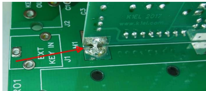
Figure 18 – Poor bridging attempt
