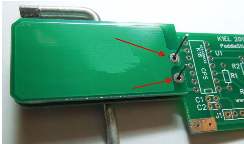
Figure 8 – Insert leads into the paddle connection hole
