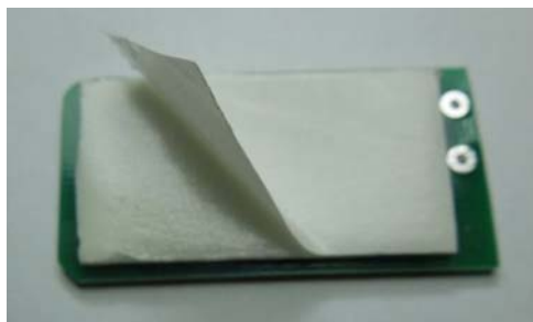
Figure 6 – Remove foam tape paper film
