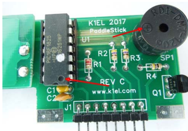
Figure 14 – Install speaker, transistor Q1, and U1
